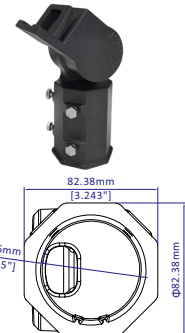
Slip Fitter Mount
