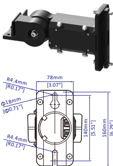
Universal bracket
