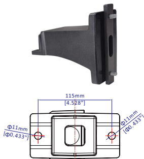
Square & Round Pole Mount
