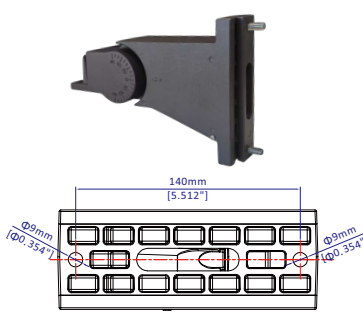
Adjustable Square & Round Pole Mount
