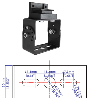
Trunnion Mount
